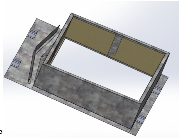
pc-2mb-1 with diverter shown (rib caps welded)
