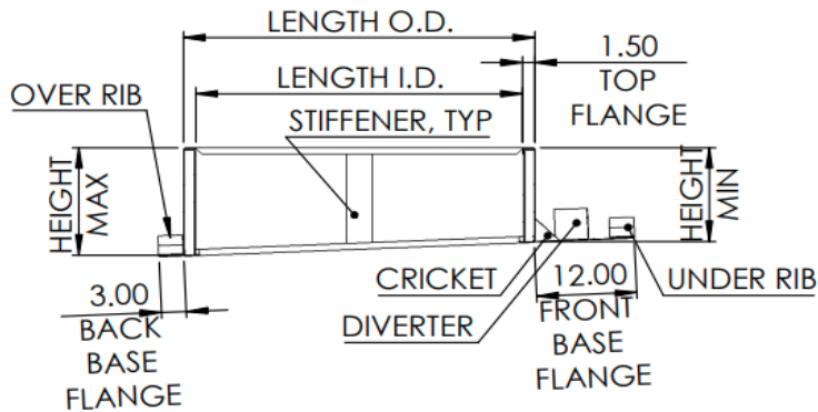
one piece curb with flat flange:
